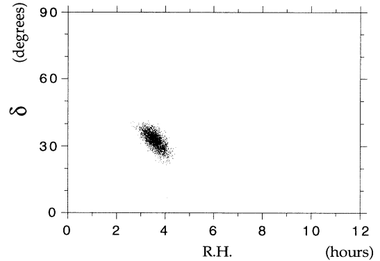
FIG. 1. Scatter plot of reconstructed positions of a source located at right ascension = 3 h, 35 min and declination \delta = 32^\circ 18' over 3000 attempts. The incoming gravitational pulse is assumed linearly polarized with polarization angle \psi = 30^\circ , the estimate of which has the same accuracy as the other two angles. The R_{SN} 's of the 6 antennae, due to their different figure pattern, are respectively 4.5, 6, 1, 9, 10, and 1.
